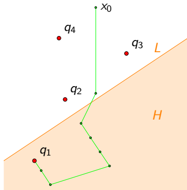
Fig. 1 A Douglas–Rachford iteration in ^2 with the set Q = \{q_1, q_2, q_3, q_4\} finds a solution in eight iterations .
