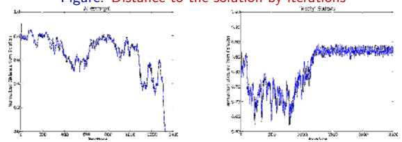
Figure. Distance to the solution by iterations
