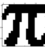
The number \pi .
