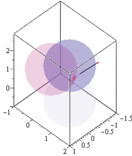
Fig. 2 Douglas-Rachford for three spheres in three-space.
