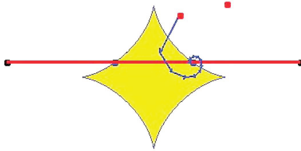
Fig. 9 Spiralling with the 1/2-sphere.
