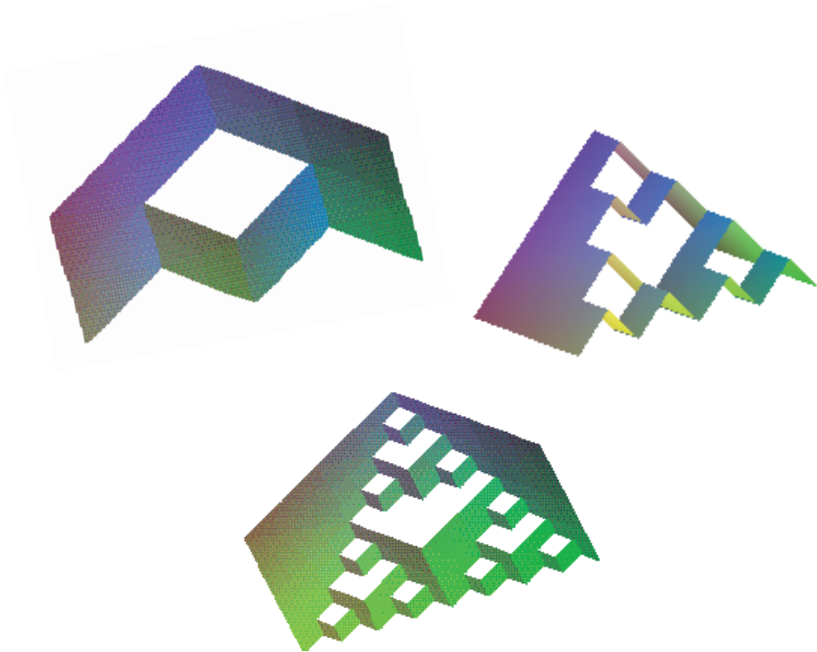
The 1st, 2nd and 3rd iterates
