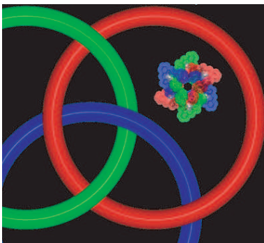
Molecular Borromean Rings
