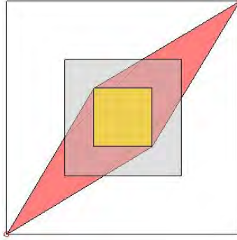
B' (red), \alpha B_{X^*} (yellow) and 2\alpha B_{X^*} (grey)
